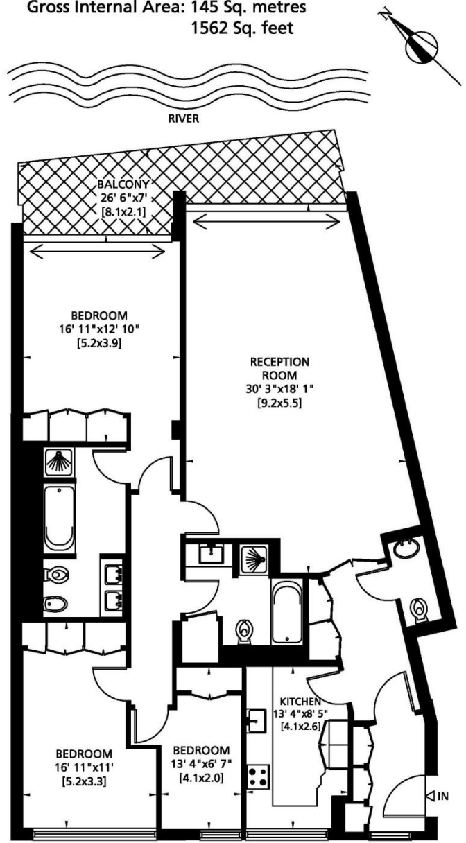
THIRD FLOOR
